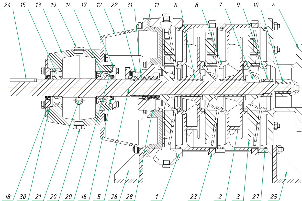
NC.3-76R1.Riflon (4" x 3" x 12") Centrifugal pump. Structure.
